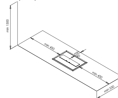
Without fire box (insert) One burner
